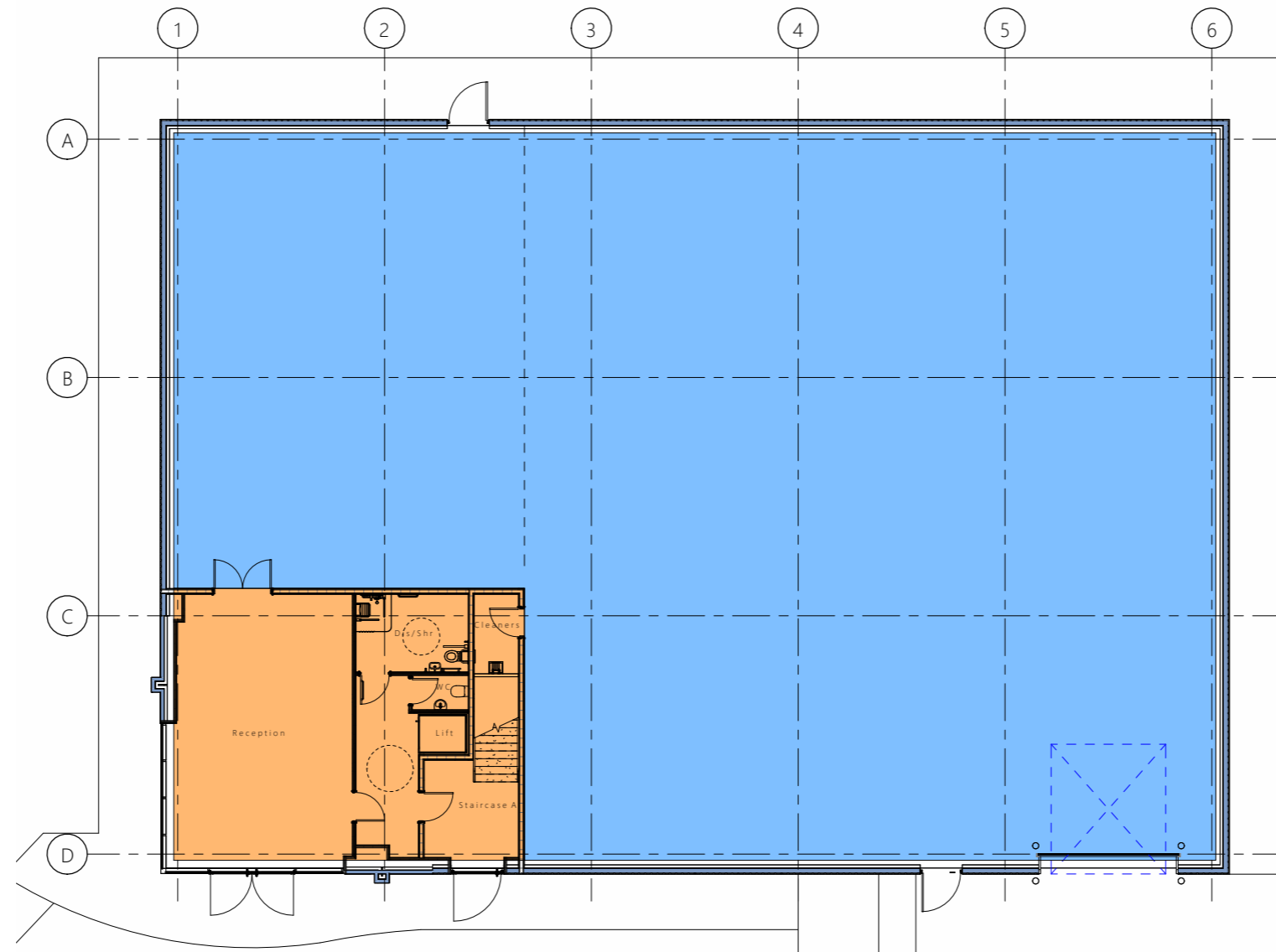
Fig. 3 Unit E Ground Floor Plan
